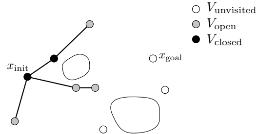
(b) Lines 4–5: given a neighboring node x , FMT* finds the neighbors of x within V_{\text{open}} and searches for a locally-optimal one-step connection. Note that paths intersecting obstacles are also lazily considered.
