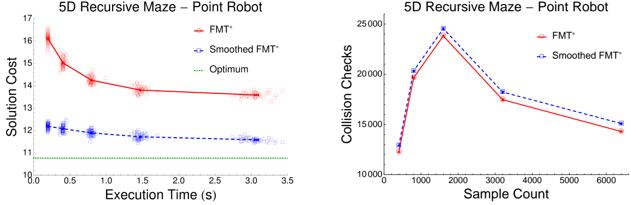
Figure 16: Simulation results for a maze configuration in 5D space.
