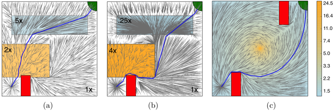
Figure 17: Planning with general costs.
